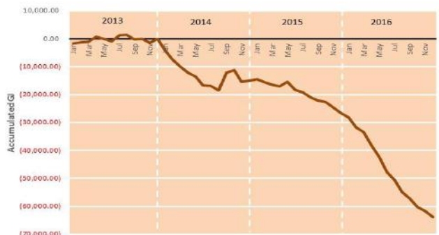
Figure 8: CUSUM Plot from 2013 – 2016 for PTTGC12
