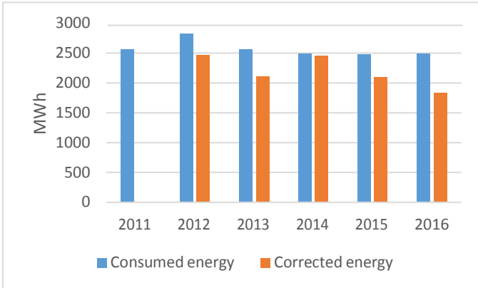
Figure above shows absolute electricity consumption (blue) and corrected values (orange) because of occupied building surface increase and degree-days compared to base line (2011).
